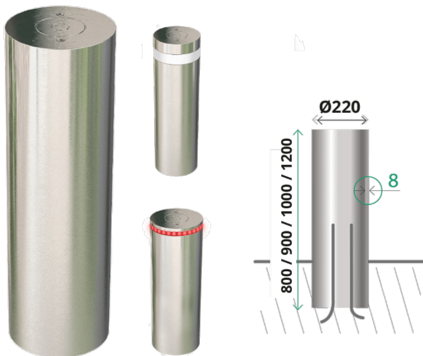
Security Fixed Ø220 HS1200
