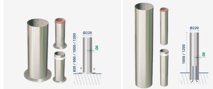
Fixed with base plate Ø220 HP220
